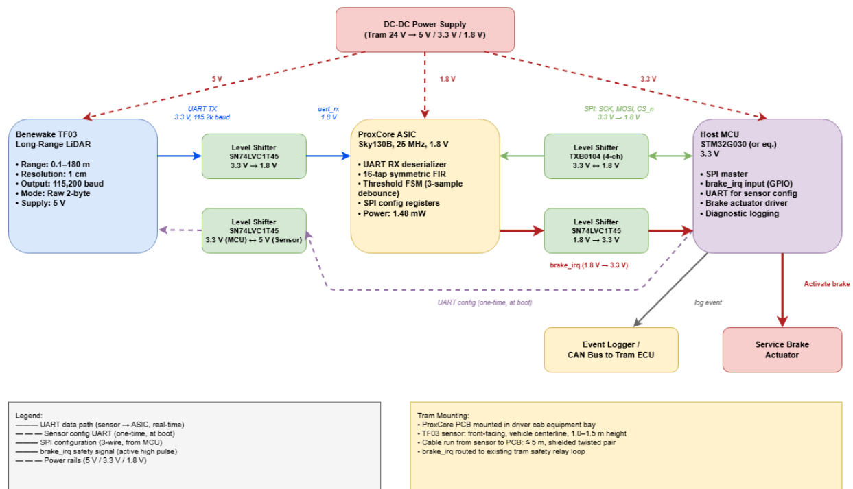
Figure 7: Urban Tram System Integration with ProxCORE
