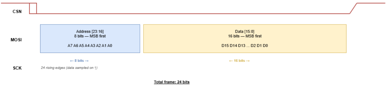
[FIGURE 2: SPI Frame Format]
